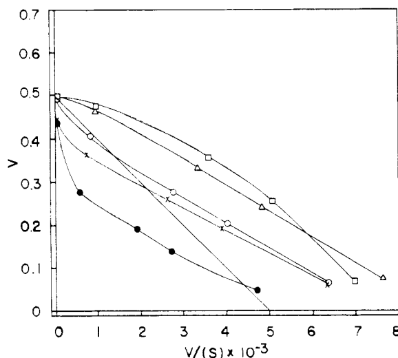
FIG. 2.—Velocity is plotted versus velocity divided by the substrate concentration for an inhibited system when the following parameters are constant: \bar{K}_1 = 1.0 \times 10^4/\text{M} , k_2 = 1.5 \times 10^4 , k_{-1} = 0.5 , k_2 = 1.0 , r = 2.0 , \bar{K}_1 = 1.0 \times 10^4/\text{M} , k'_1 = 1.0 \times 10^4 , k'_{-1} = 1.0 , k'_2 = 0.0 , r' = 0.0 , (I)K_0 = 1.0 , (I)K'_0 = 1.0 .
